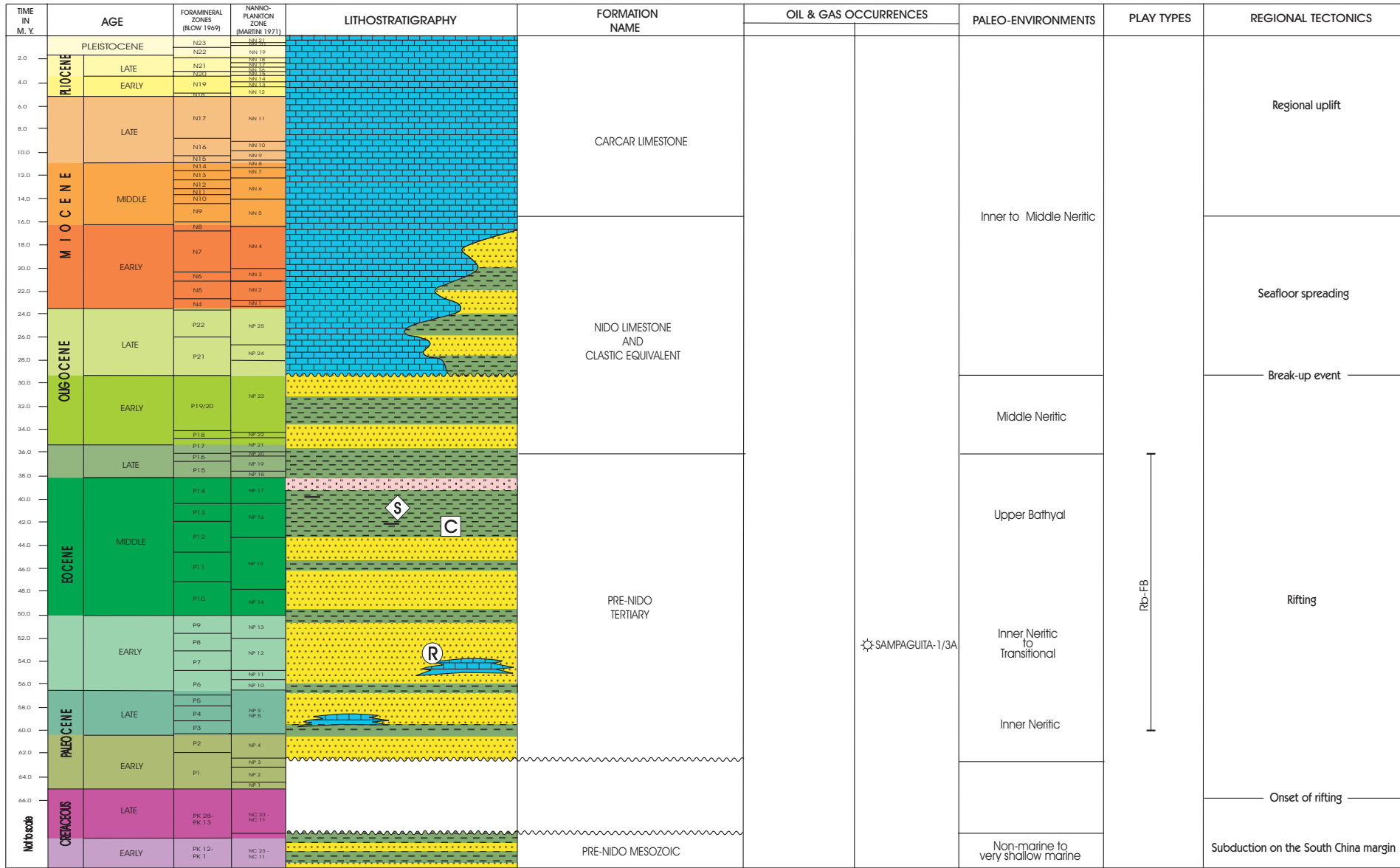
Stratigraphic Column of the Reed Bank Basin
