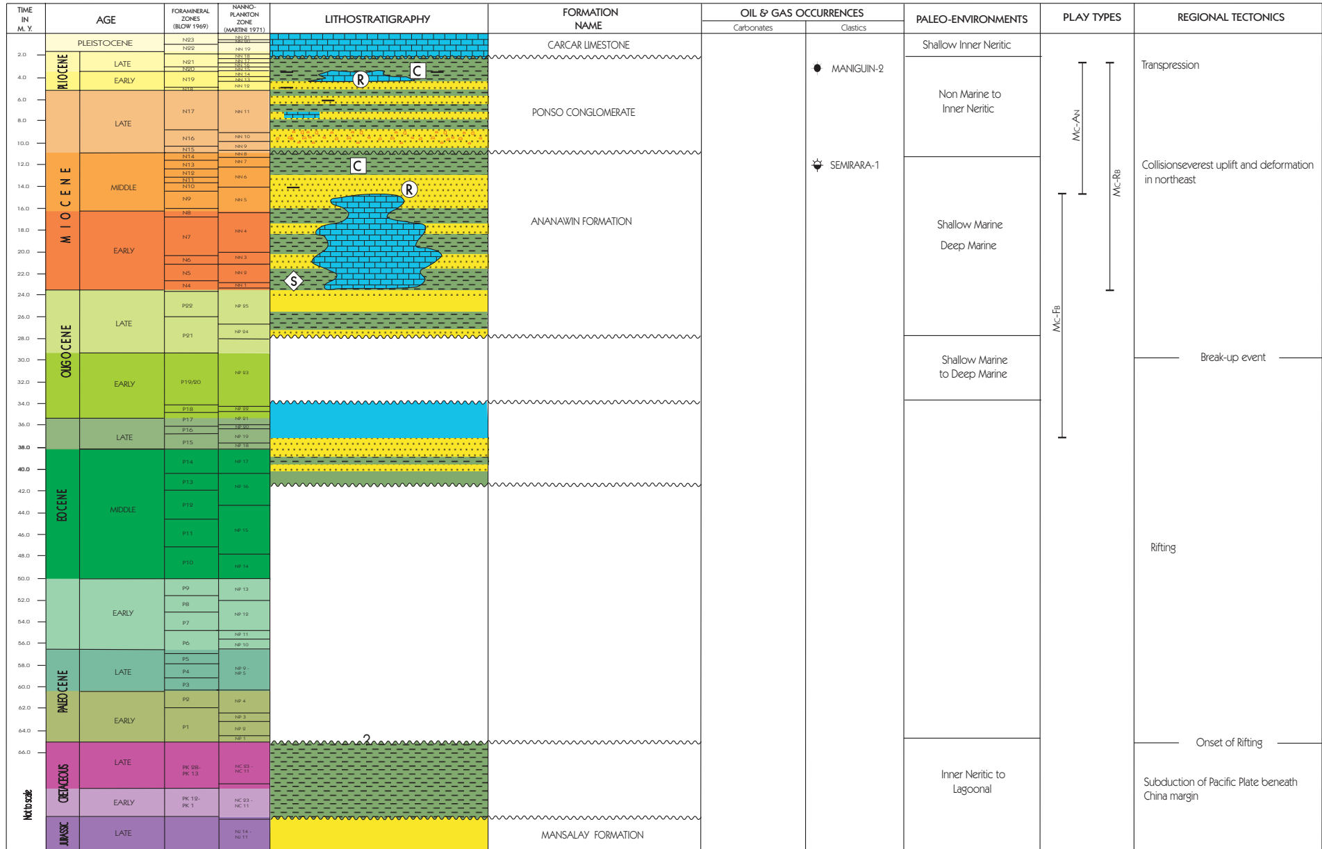
Stratigraphic Column of the Mindoro - Cuyo Basin
