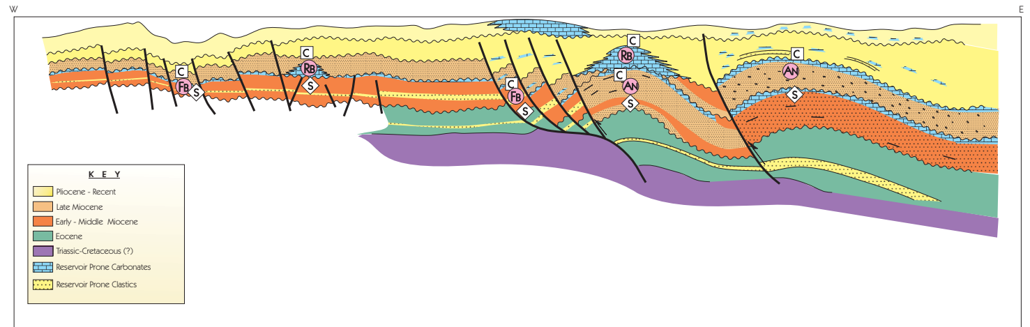
Schematic Play Concept Diagram for the Petroleum System in the Mindoro-Cuyo Basin
