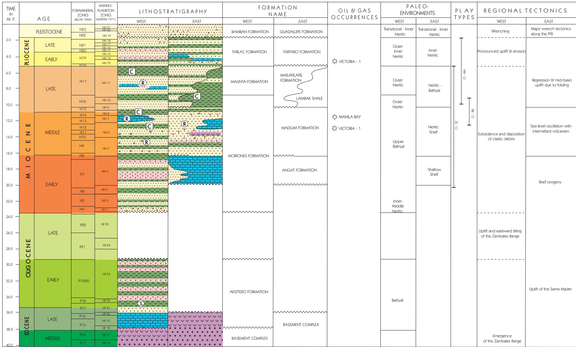
Stratigraphic Column of the Central Luzon Basin
