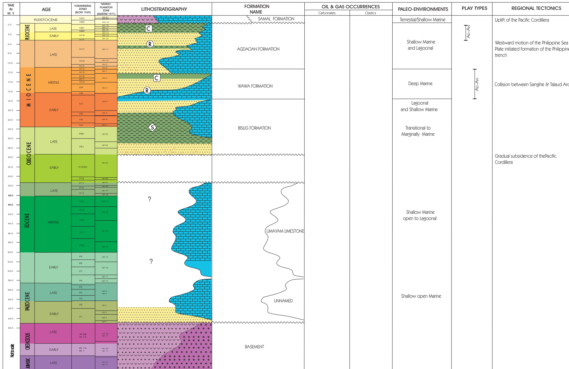
Stratigraphic Column of the Agusan-Davao Basin
