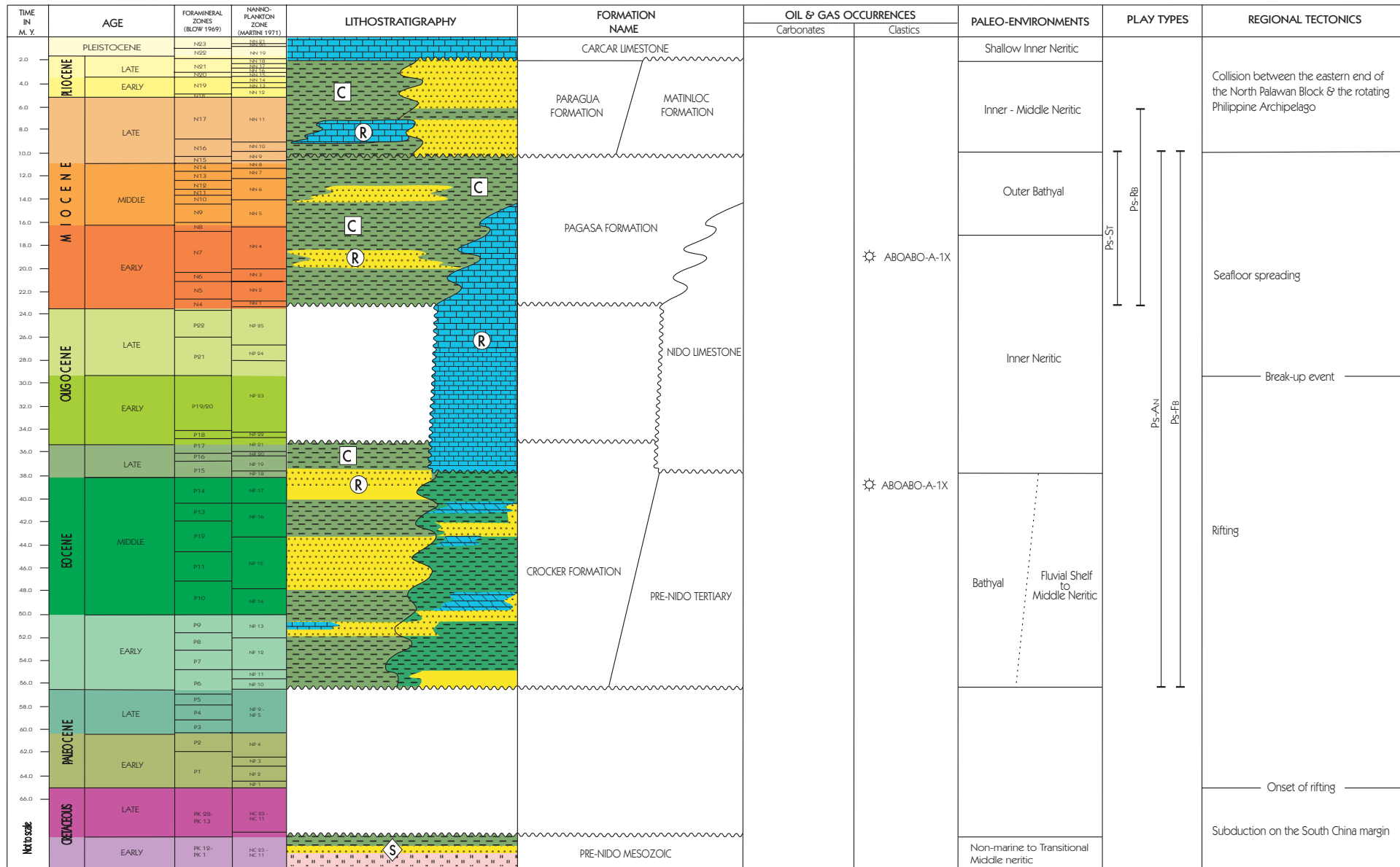
Stratigraphic Column of the Southwest Palawan Basin
