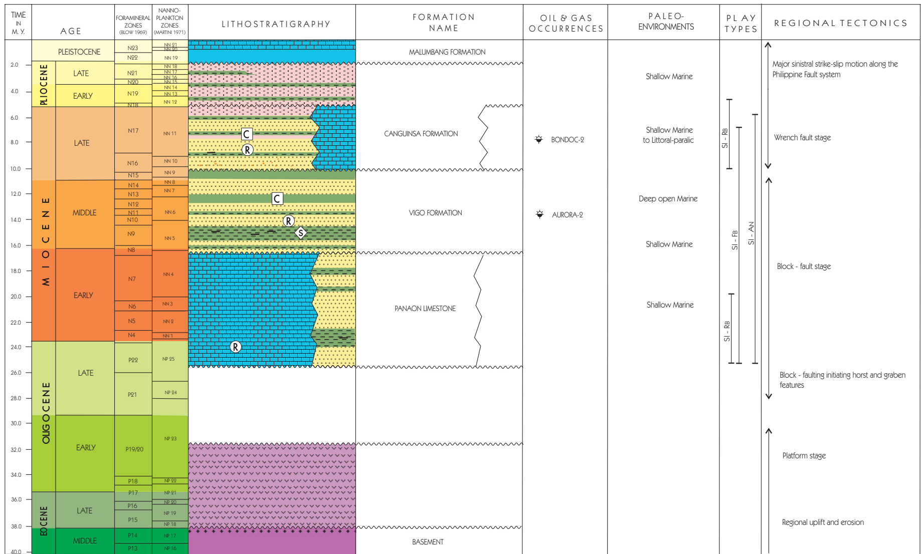
Stratigraphic Column of Southeast the Southeast Luzon Basinl (Bondoc Peninsula)
